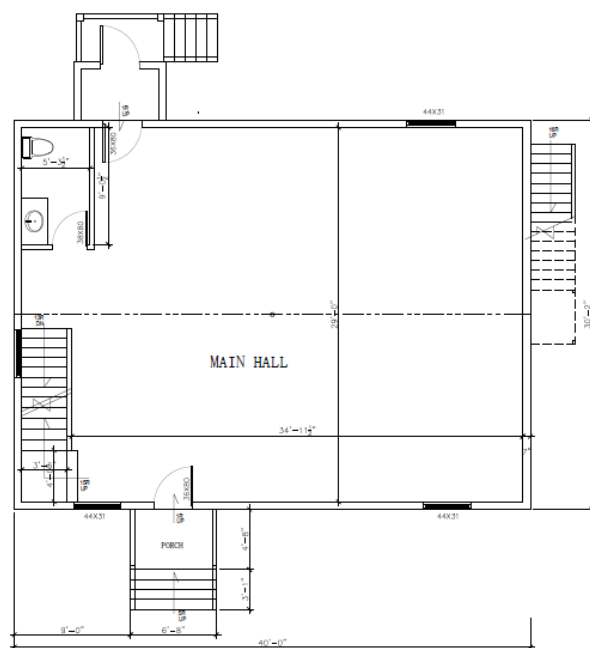
EXISTING MAIN FLOOR PLAN 1/8"=1'
