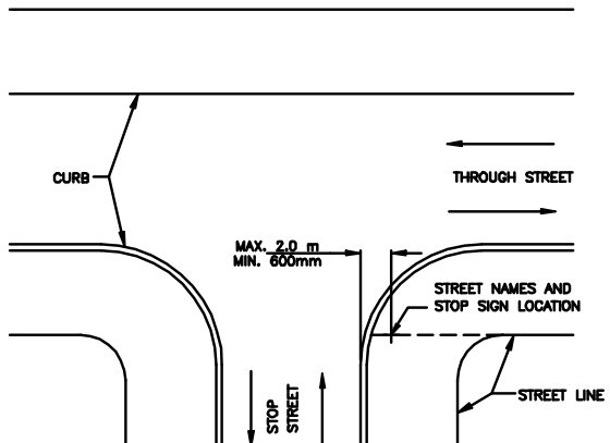
3 WAY INTERSECTION
