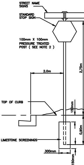
STREET SIGNS AND STOP SIGN DETAILS
