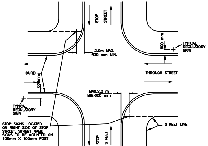
4 WAY INTERSECTION
